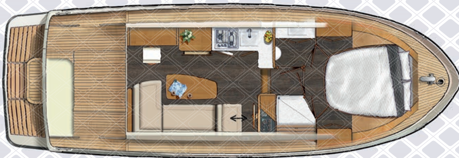
Layout Linssen 30 SL Sedan
